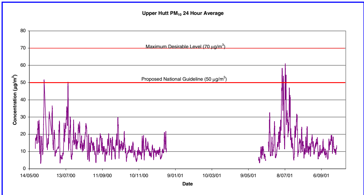
Figure 4.9 24-Hour Moving Average PM 10 (µg/m 3 ) at Trentham Fire Station from 22/5/00 to 1/10/01
