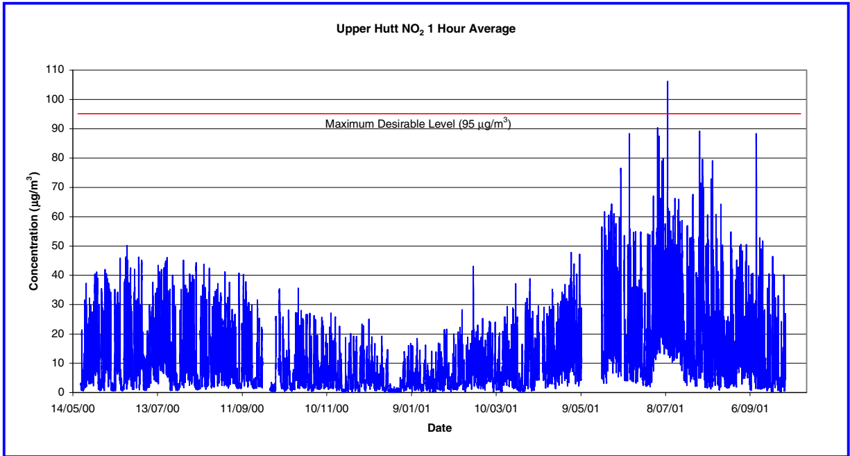
Figure 4.4 1-Hour Moving Average NO 2 (µg/m 3 ) at Trentham Fire Station from 19/5/00 to 1/10/01
