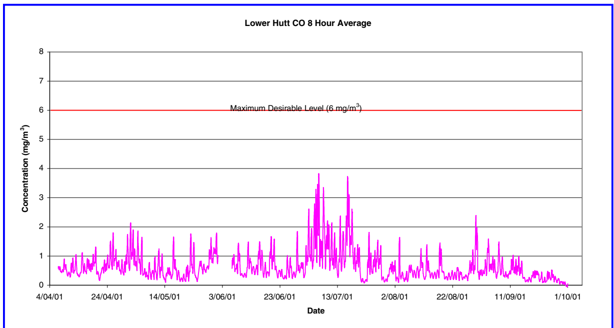
Figure 4.24 8-Hour Moving Average CO (mg/m 3 ) at Birch Lane from 5/4/01 to 1/10/01
