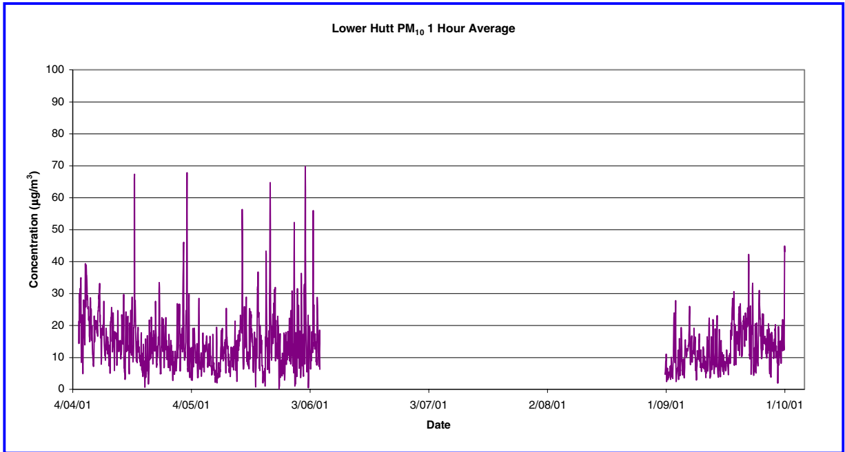
Figure 4.20 1 Hour Moving Average PM 10 (µg/m 3 ) at Birch Lane from 5/4/01 to 1/10/01
