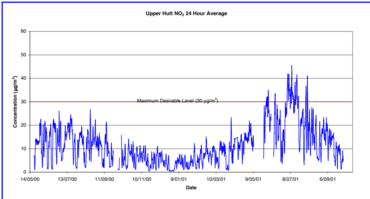
Figure 4.5 24-Hour Moving Average NO 2 (µg/m 3 ) at Trentham Fire Station from 19/5/00 to 1/10/01
