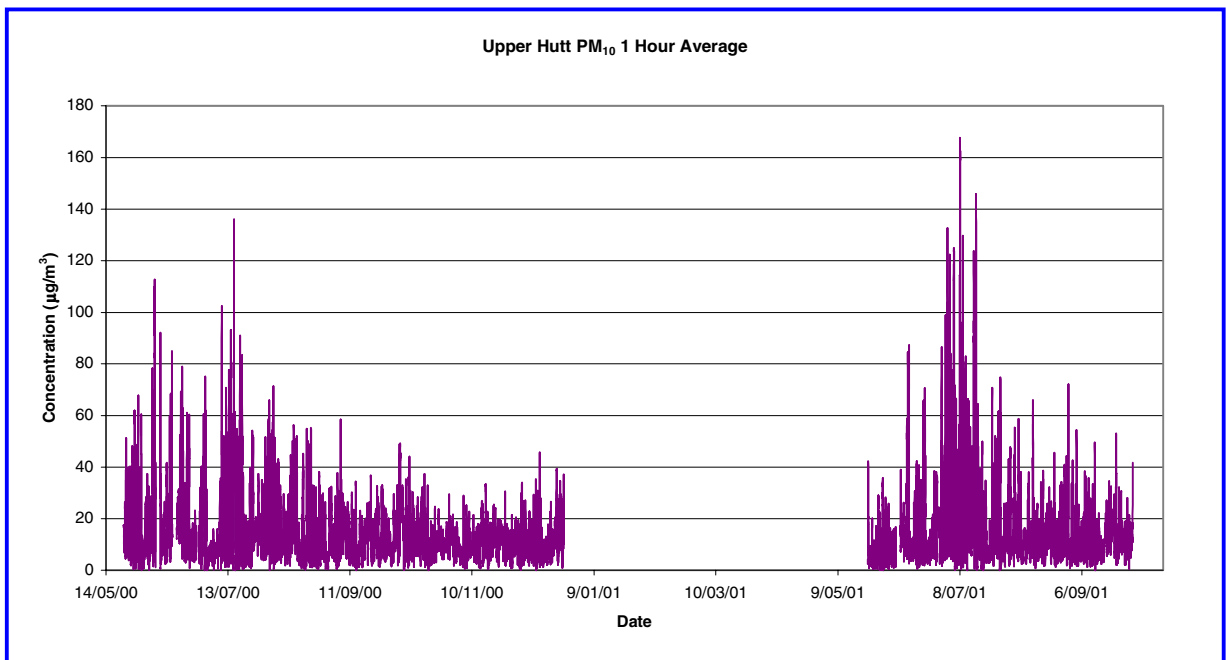
Figure 4.8 1 Hour Moving Average PM 10 (µg/m 3 ) at Trentham Fire Station from 22/5/00 to 1/10/01
