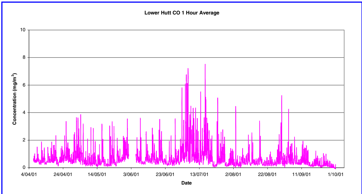
Figure 4.23 1-Hour Moving Average CO (mg/m 3 ) at Birch Lane from 5/4/01 to 1/10/01
