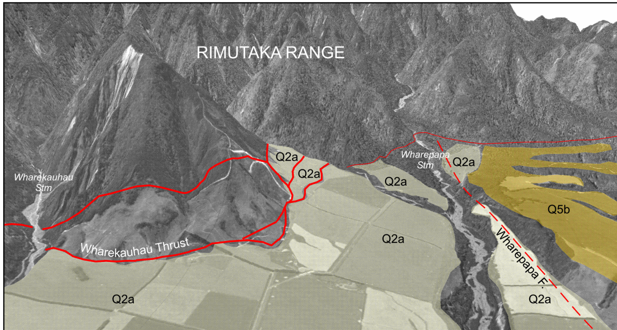
Fig. 10. Oblique elevated image of the Wharekahu Thrust from a position close to the Stop point. A vertical aerial photo is draped over a digital topographic model, with a vertical exaggeration to highlight the Wharekahu Fault. Note the lobate splays of the thrust, and its displacement of the Waiohine surface (Q2a). The Wharepapa Fault is not exposed at the surface, and probably has not been active since the Last Glaciation. Note the Waiohine surface gravels lapping against the older Quaternary deposits below the Last Interglacial marine bench in the right foreground. (Base image by J.M. Lee).
