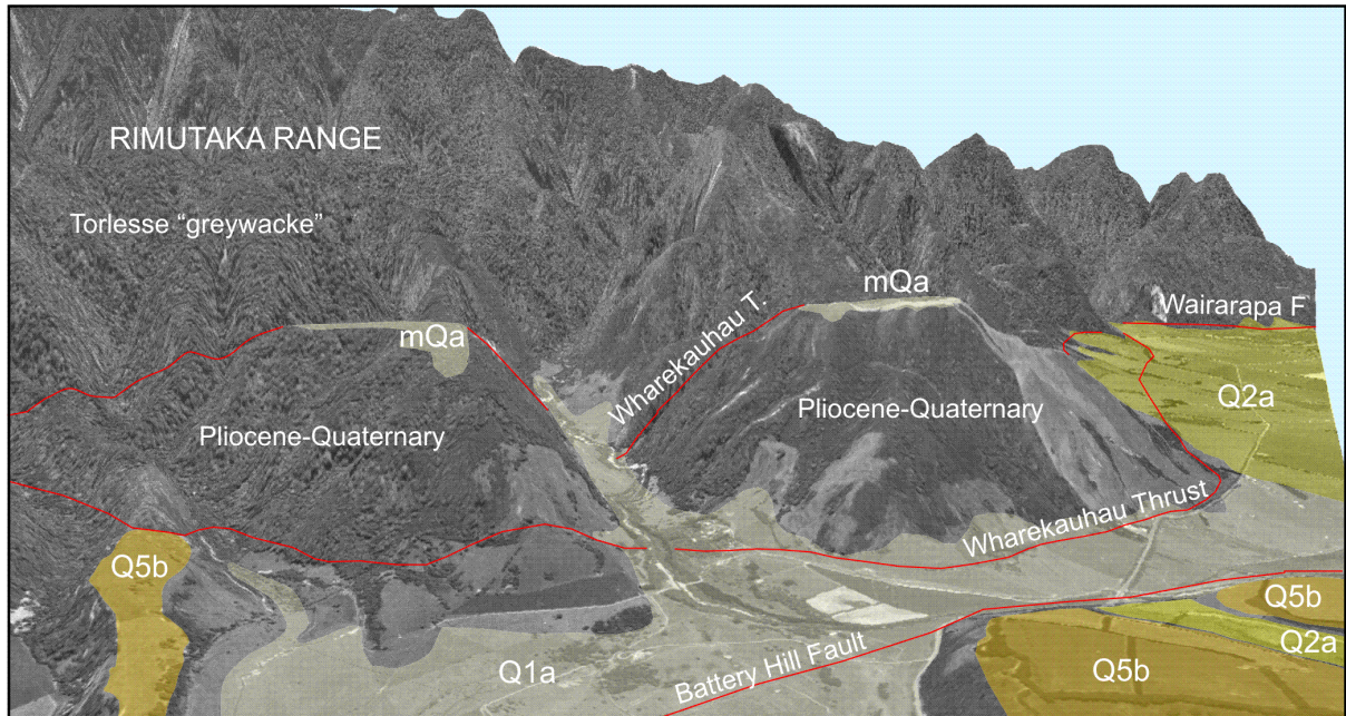
Fig. 12. Oblique elevated image of the Manganui Stream area. The vertical scale is considerably exaggerated. Note the truncation of the Last Interglacial marine bench by the Wharekahu Thrust (Q5b, left foreground) and the location of the 1855 trace across Manganui Stream (Stop 2). Note also the Pounui Anticline, capped by the raised and folded Last Interglacial marine bench. The marine bench is bisected by an abandoned Last Glacial Manganui Stream course. (Base image by J.M. Lee).
