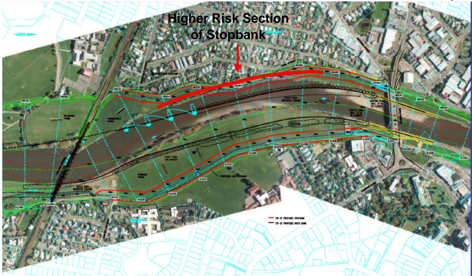
Ava to Ewen Project – Higher Risk section of Alicetown Stopbank
