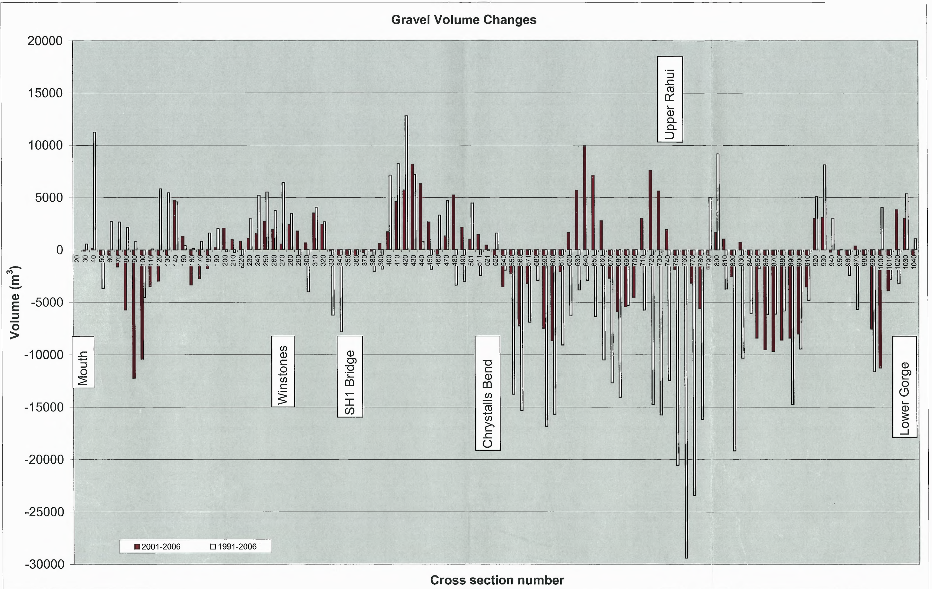
Figure: Otaki River Gravel Volume Changes.
