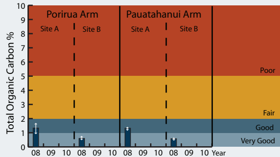
Figure 3. Total organic carbon (mean and range) at 4 intertidal sites, Jan. 2008.
