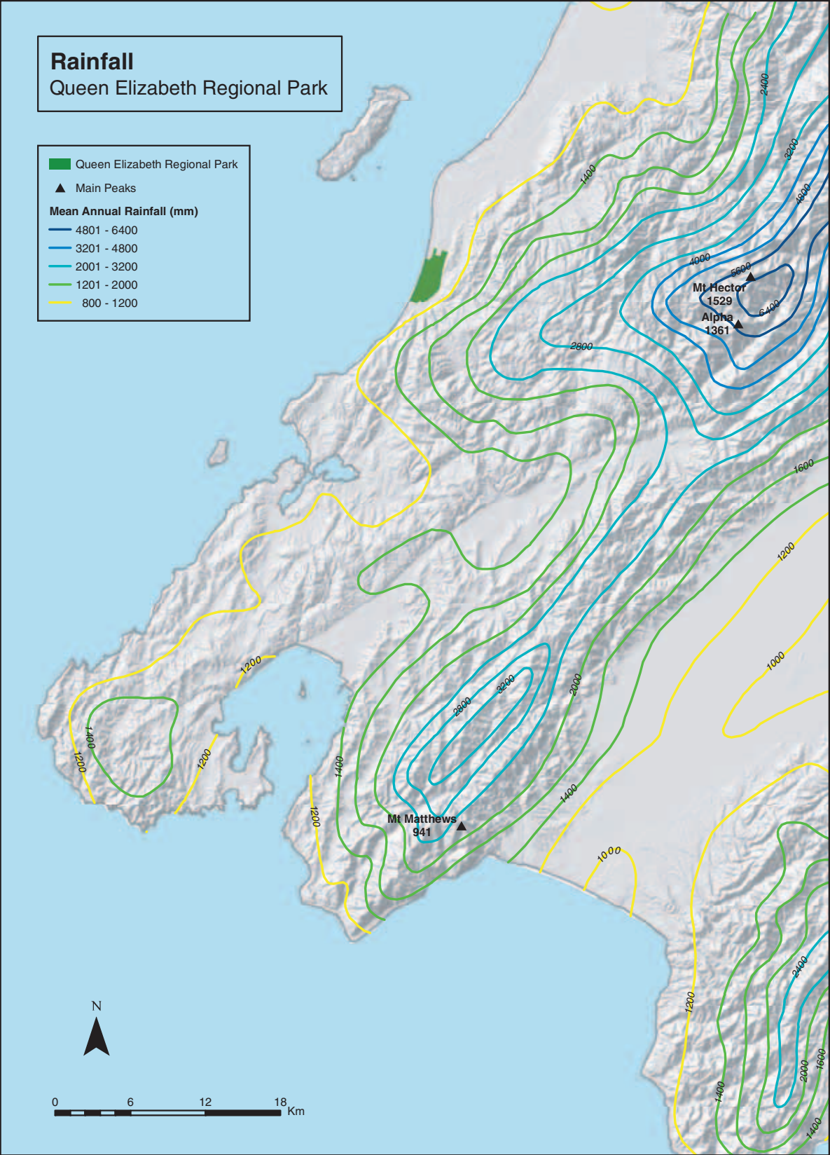
Map 4 Regional rainfall
